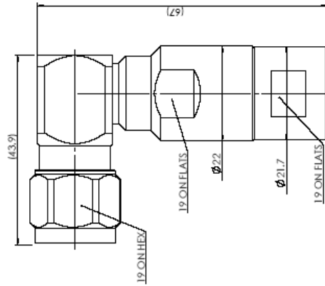
Dimensions mm
